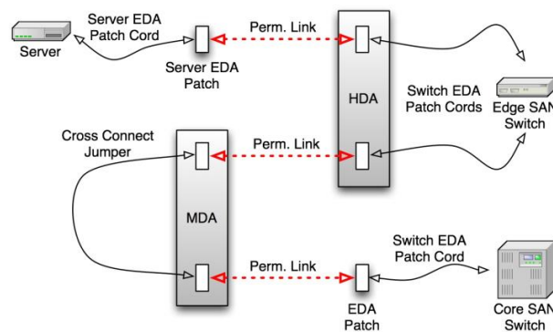
Figure 1. Storage area network cable plant permanent links (red).
