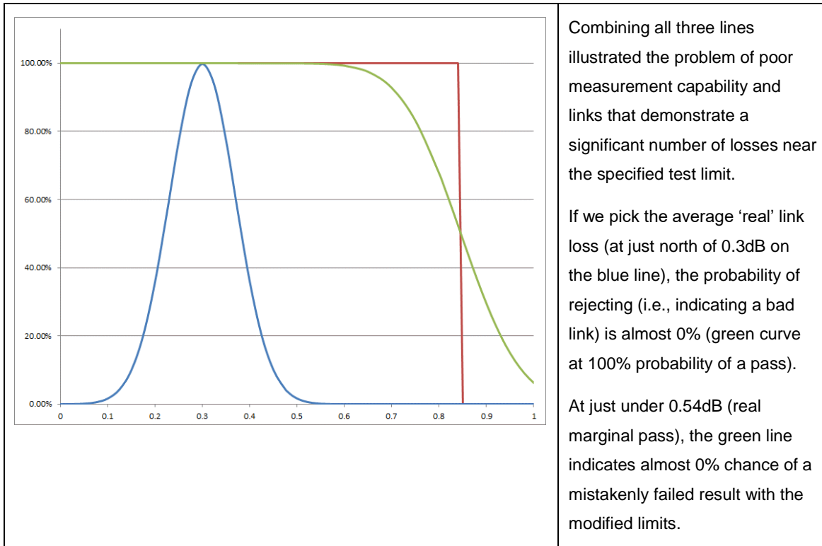
Figure 12. Guardbanded operating characteristic curve for light source/power meter.
