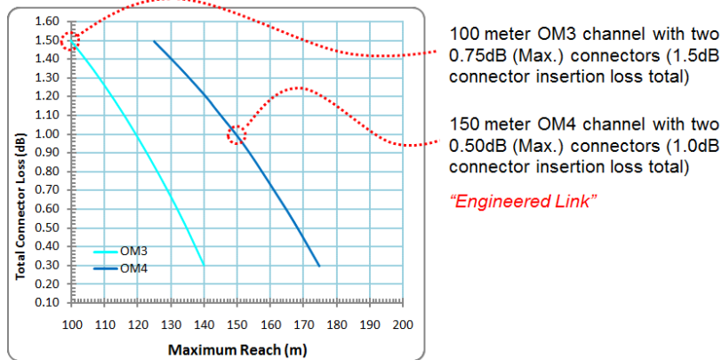
Figure 5. Extrapolation/Interpolation from IEEE model for various connector insertion loss values.
