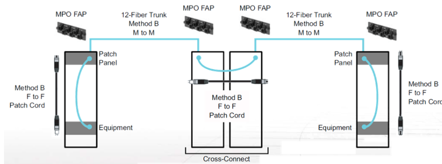
Figure 4. 40GBASE-SR4 engineered channel example.
