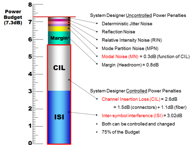
Figure 3. Optical channel budget for 10 Gb/s Ethernet (10GBASE-SR).
