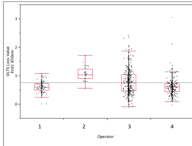
Figure 3. Box-Whisker chart of fan-out IL vs. operator (measuring same product).
