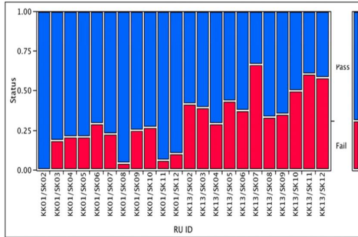
Figure 15. Plot showing link fail rate (% , in red) and link pass rate (% , in blue) vs. rack location (RU ID).
