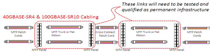
Figure 6. Parallel optics cross-connect cable plant.
