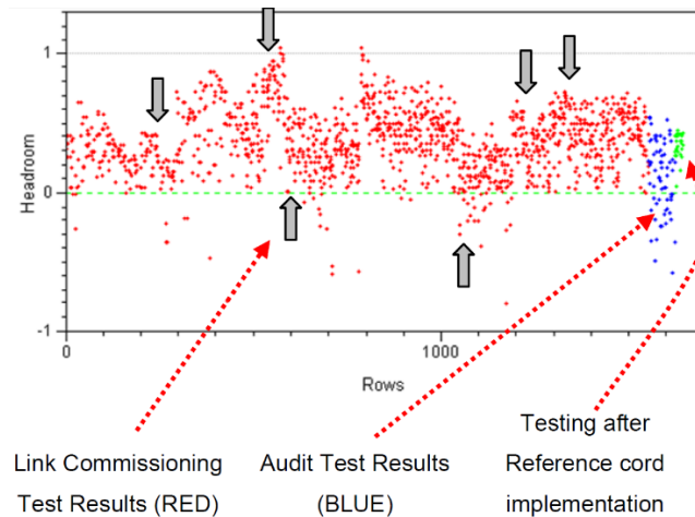
Figure 13. Headroom data.
