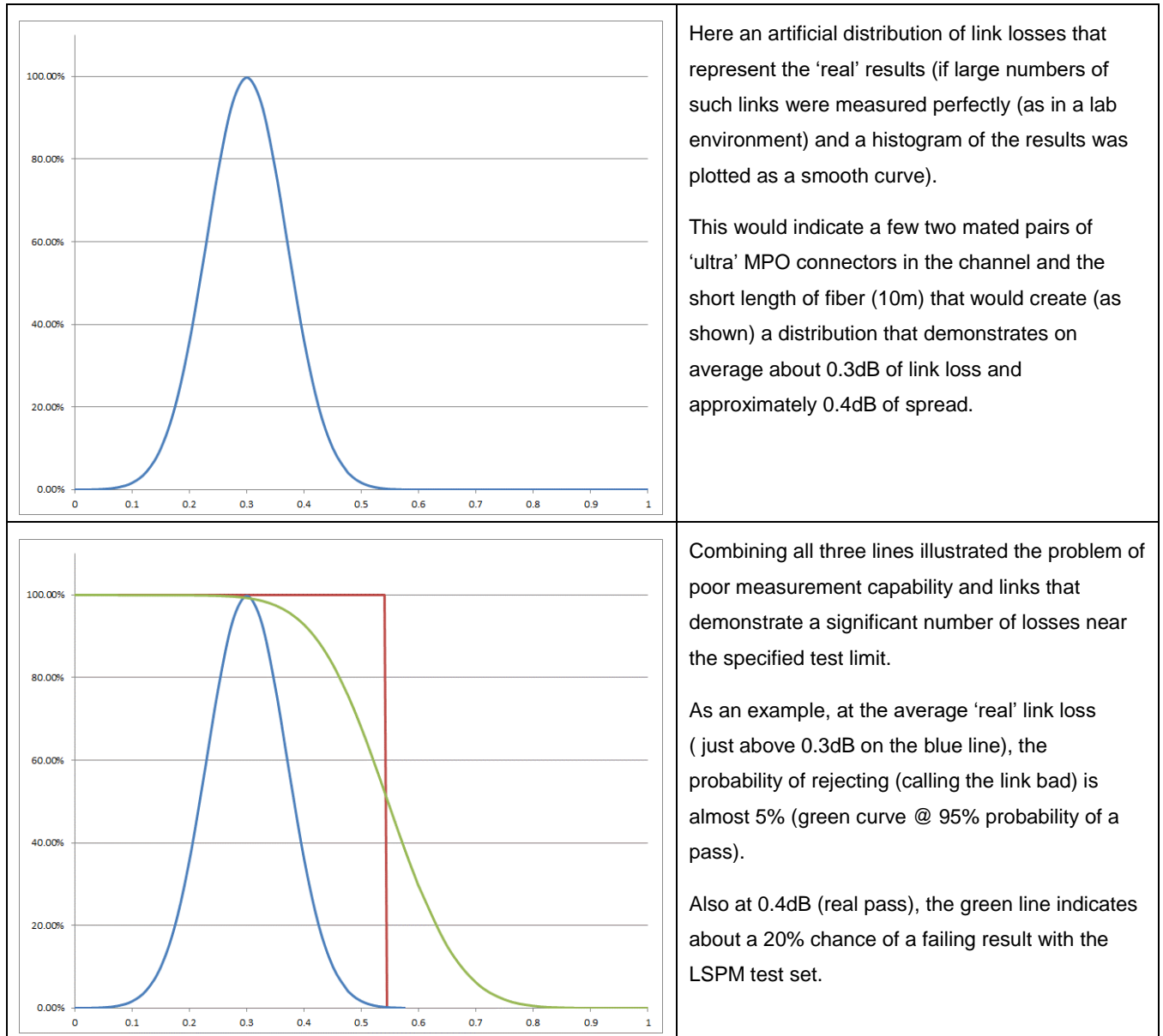
Figure 10. Operating characteristic curves for light source/power meter.
