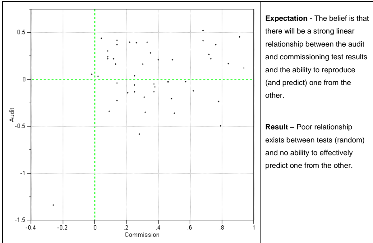
Figure 14. Plot correlating first commissioned measurements against audit results.
