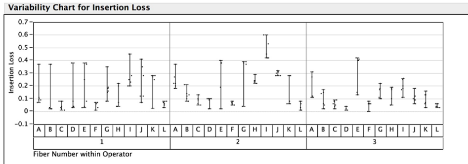
Figure 7. Sample output from a GR&R analysis on a typical LSPM.
