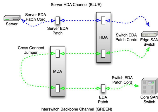
Figure 2. Storage area network cable plant channel (blue & green).
