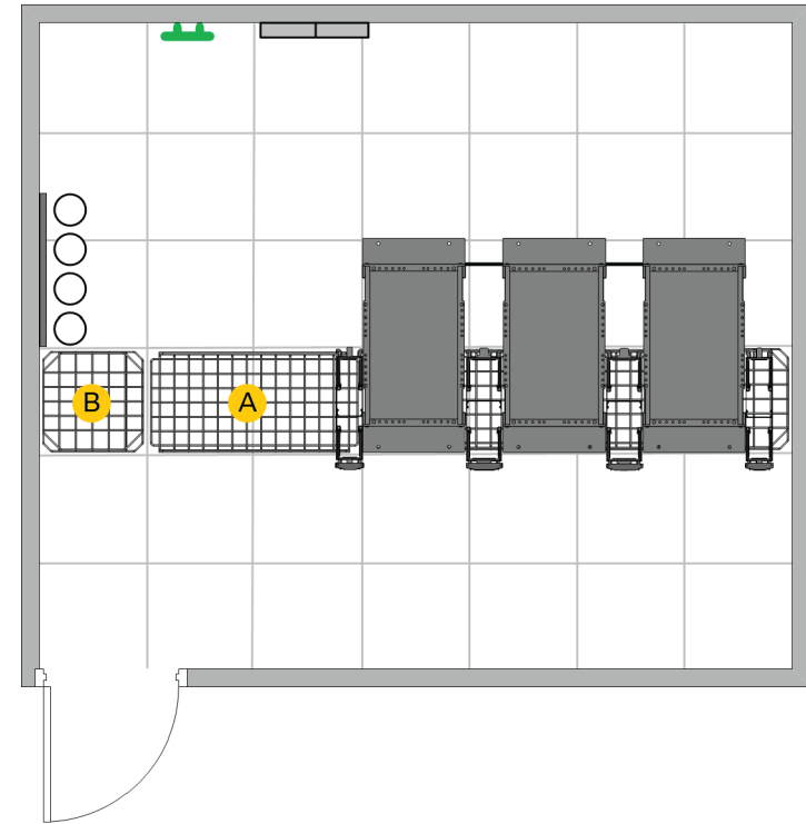
Figure 7 - Underfloor pathways within the TR
