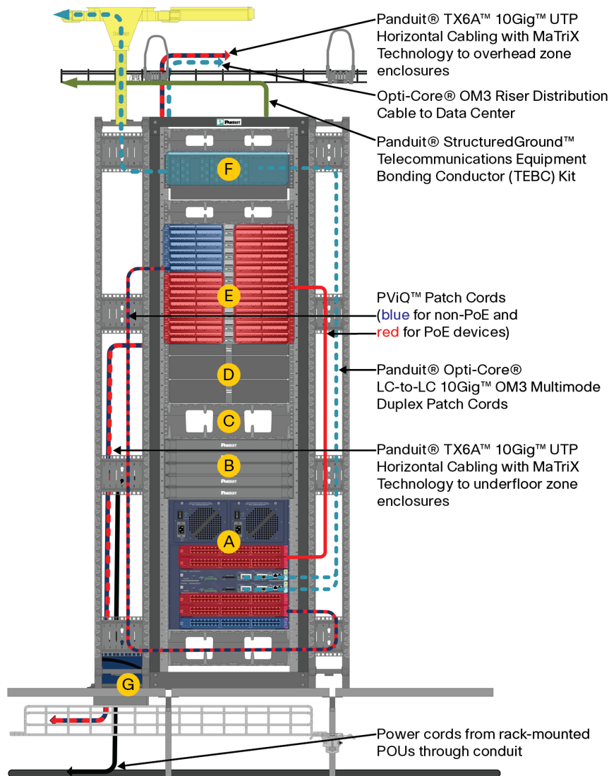
Figure 10 - Cable routing inside rack F4
