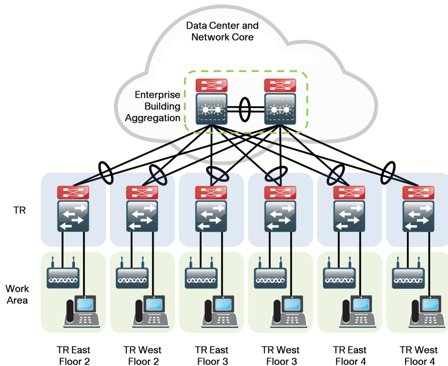
Figure 3 - Cisco SBA LAN design overview
