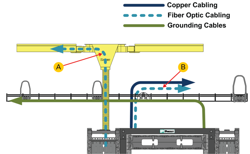
Figure 8 - Close up on overhead pathways cabling
