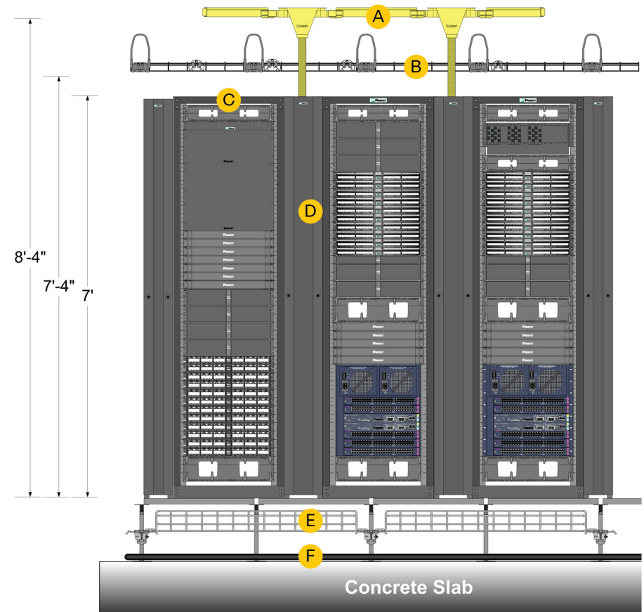
Figure 9 - Rack elevations of the TR closet
