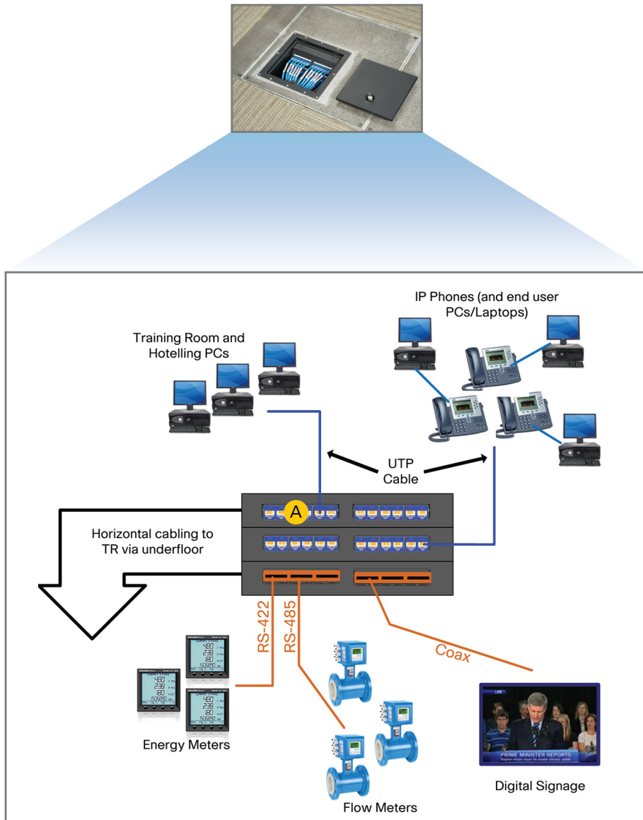
Figure 20 - PanZone® enterprise in-floor enclosure
