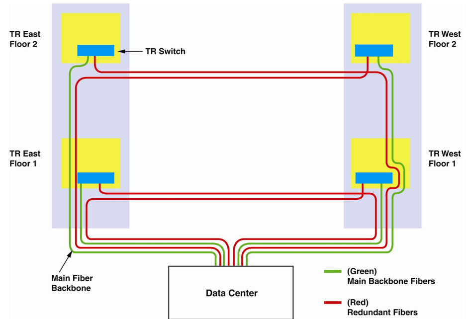
Figure 2 - Schematic arrangement for telecom rooms on two floors
