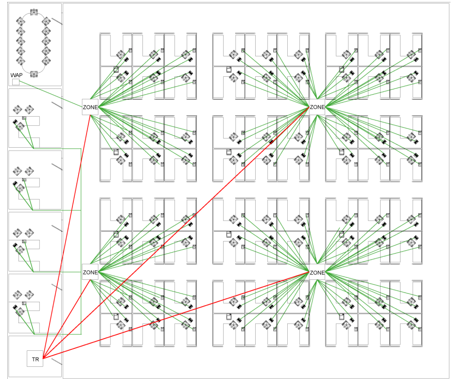
Figure 19 - Summary of zone cabling architecture
