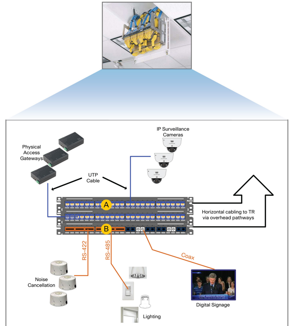
Figure 21 - PanZone® passive in-ceiling enclosure
