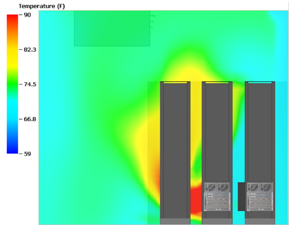
Figure 16 - Cross-sectional view of the temperature distribution—exhaust duct
